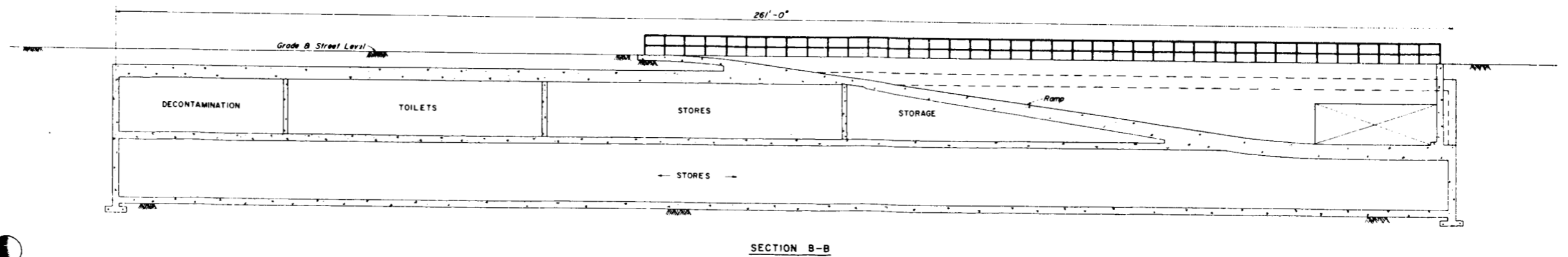
Fig. 3—Preliminary layout of prototype flat-slab structure.
